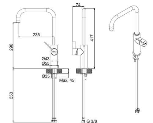
Faucet Dimensions
